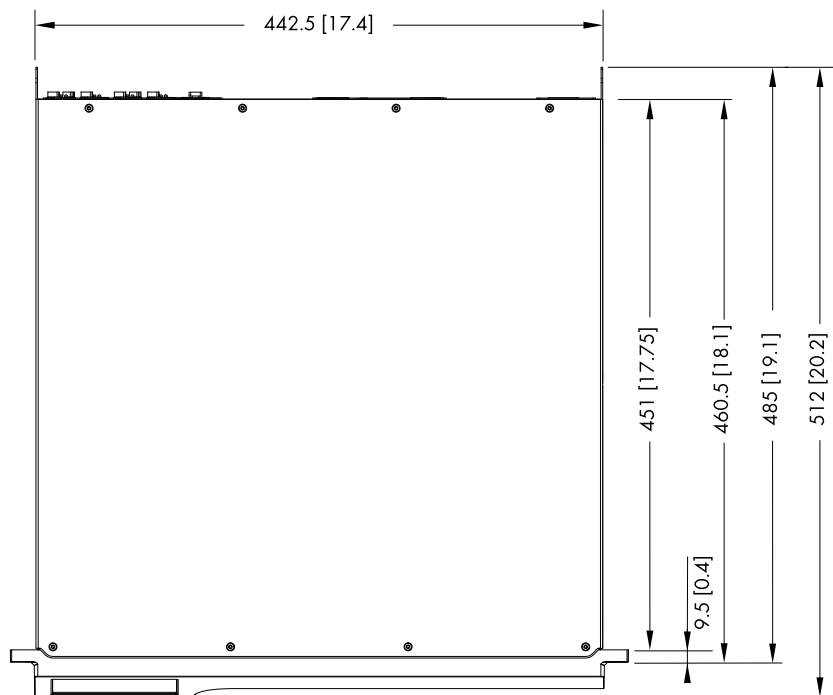
D40 dimension in mm [inch]
