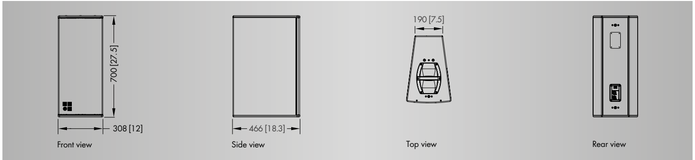
V7P cabinet dimensions in mm [inch]
