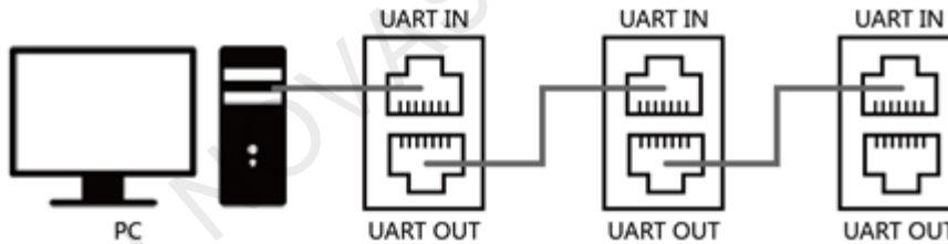
Figure 4-1 Cascading devices
