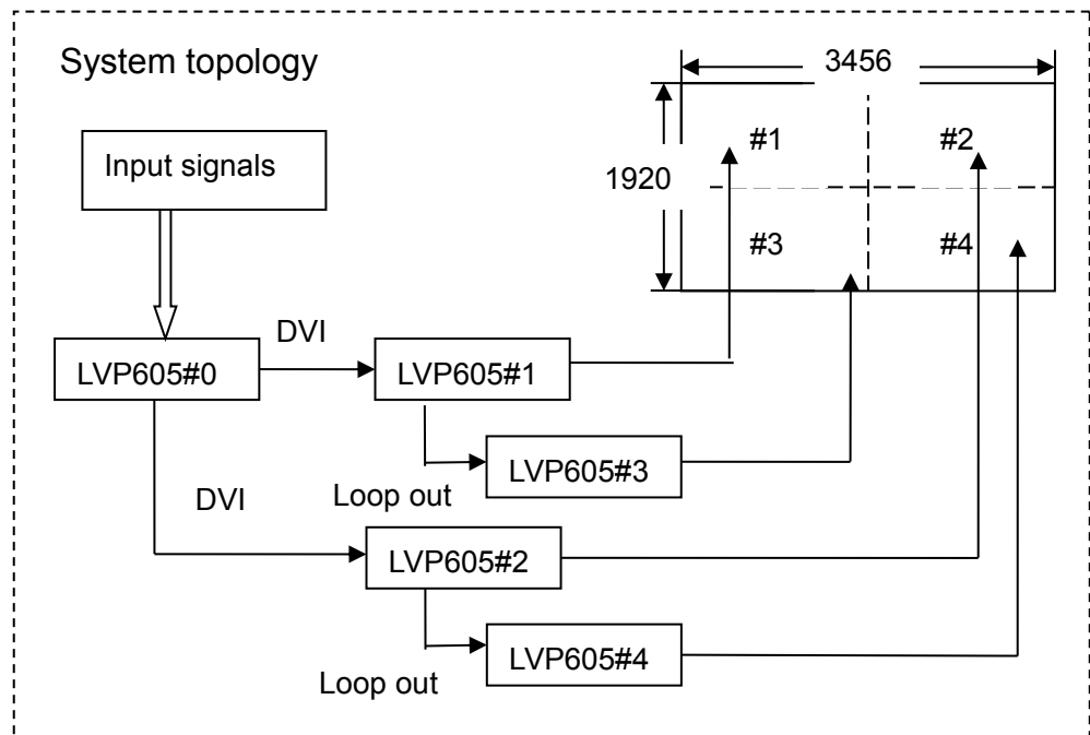
Figure 5-5 system topology
