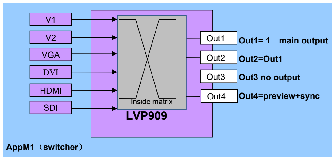
Pic 5-1A LVP909 application mode 1 sketch map
