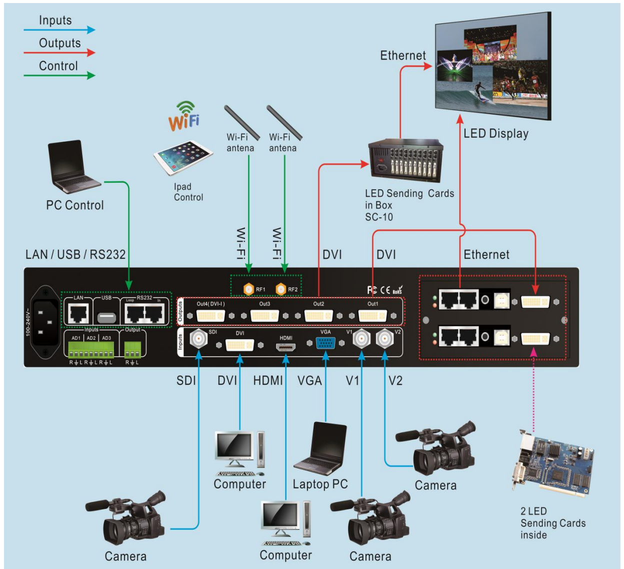
Pic 3-2 hardware connection diagram
