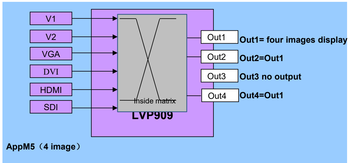
Pic 5-5a LVP909 application mode 5 sketch map
