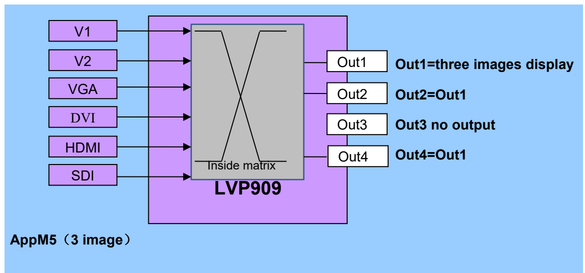
Pic 5-6a LVP909 application mode 6 sketch map
