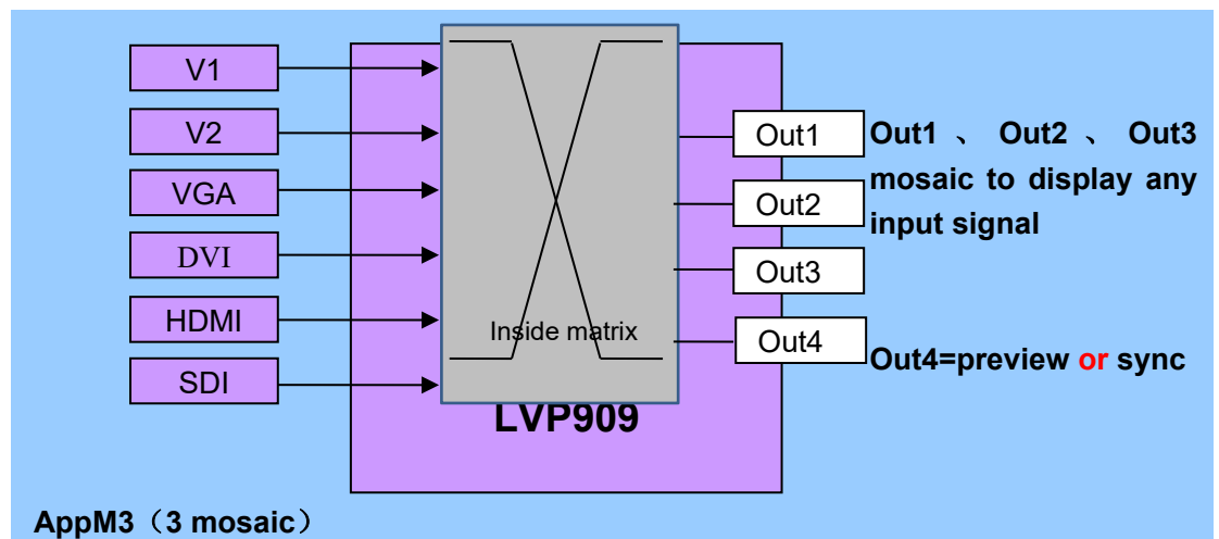
Pic 5-3a LVP909 application mode 3 sketch map
