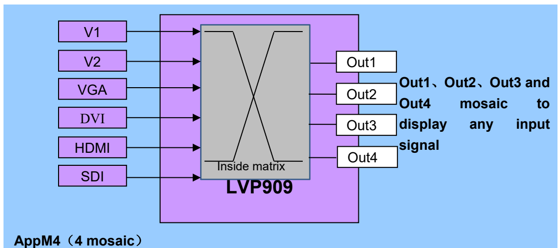
Pic 5-4a LVP909 application mode 4 sketch map
