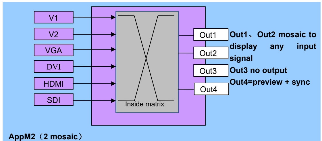
Pic 5-2a LVP909 application mode 2 sketch map
