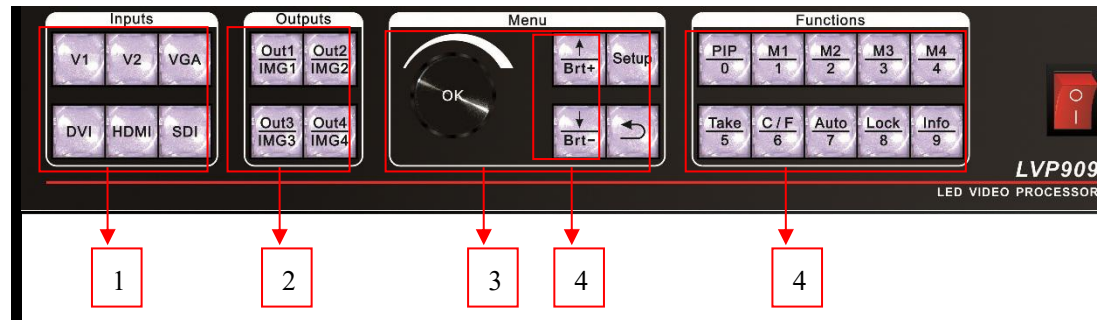
4-1 Front Panel Buttons Schematic
